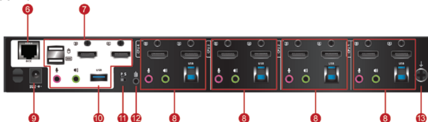
GCS1944H Back View
