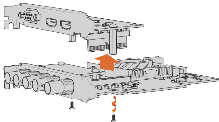
Mezzanine cards can easily be removed and attached
