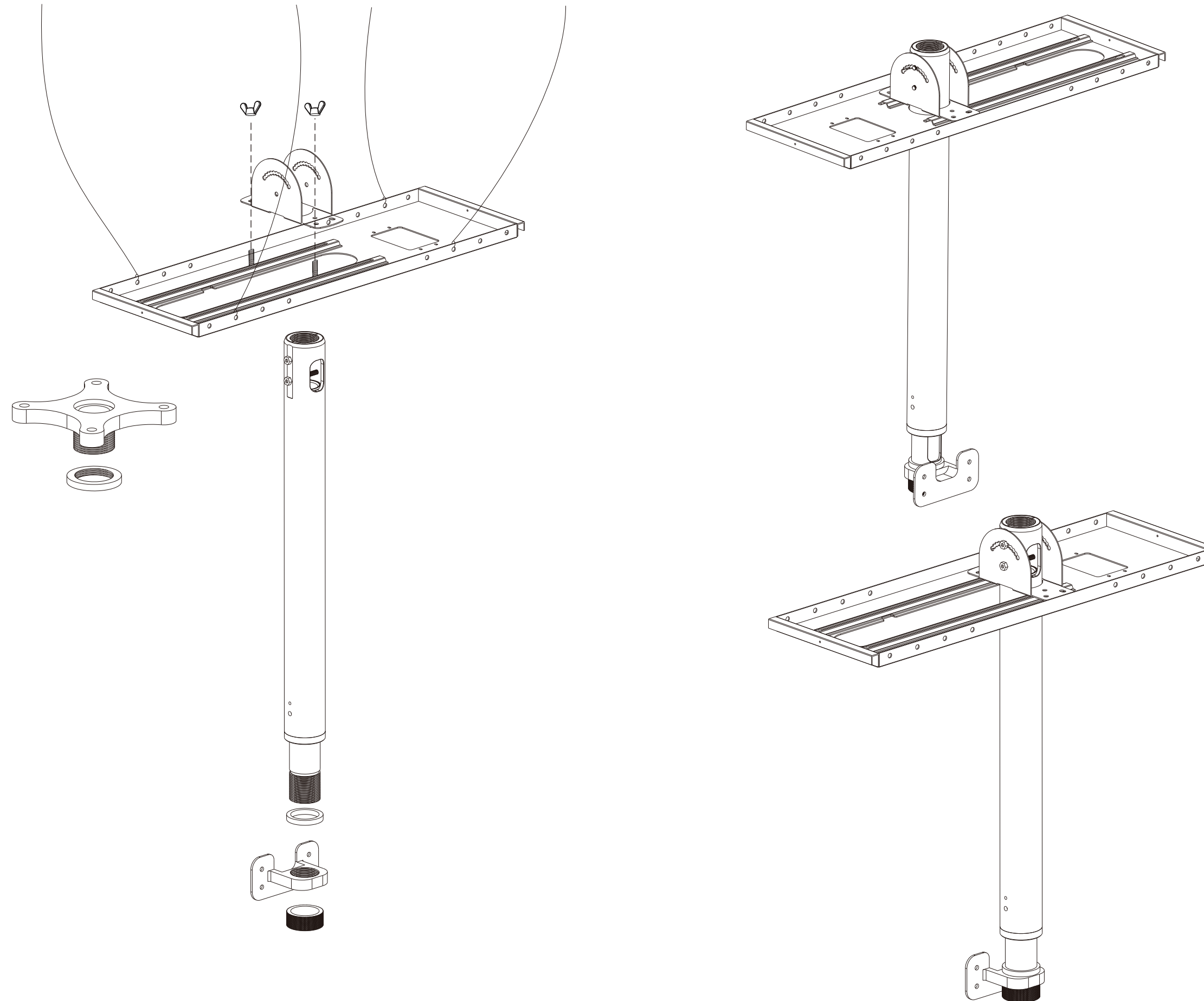
Drop Ceiling Pendant Mount Set (In Box) - (Wall Mount Not Included)
