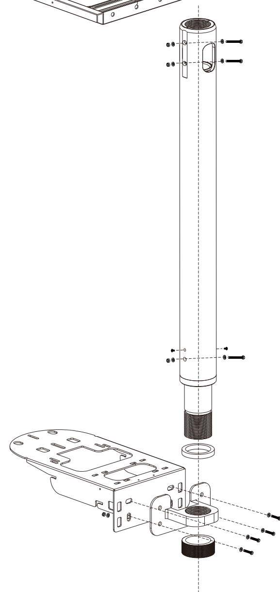
Product Configuration A Drop Ceiling Pendant Mount Set + Wall Mount Bracket (3 Sizes)
